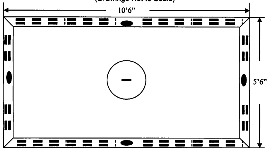
TOP VIEW-TOP 1 CLEANOUT - 24" DIAMETER
