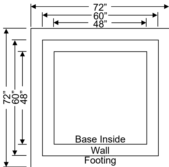
Top View-Inside
