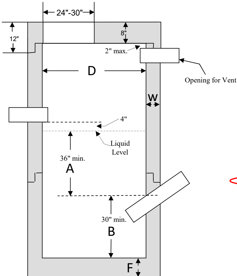
Section View - Typical Installation
