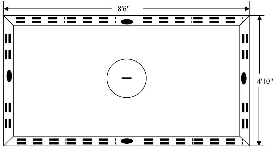
TOP VIEW-TOP 1 CLEANOUT - 24" DIAMETER
